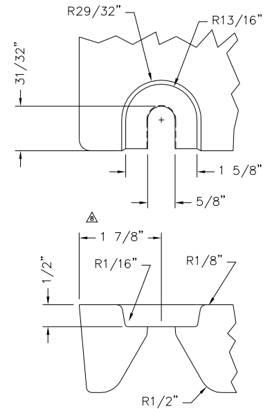
BOLT SLOT DETAIL
